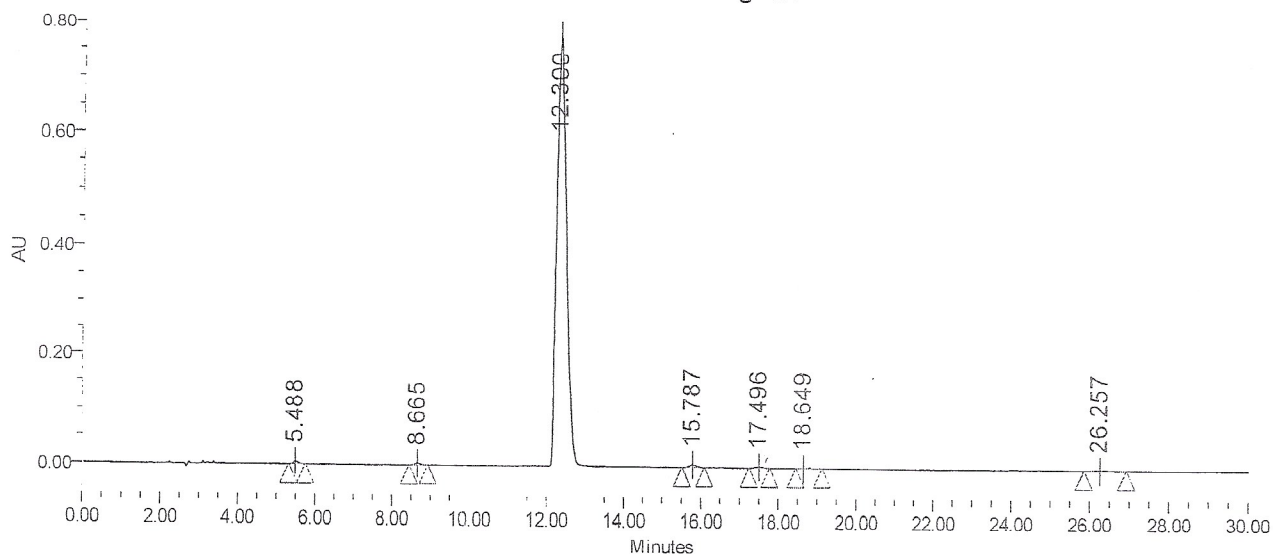
Auto-Scaled Chromatogram
